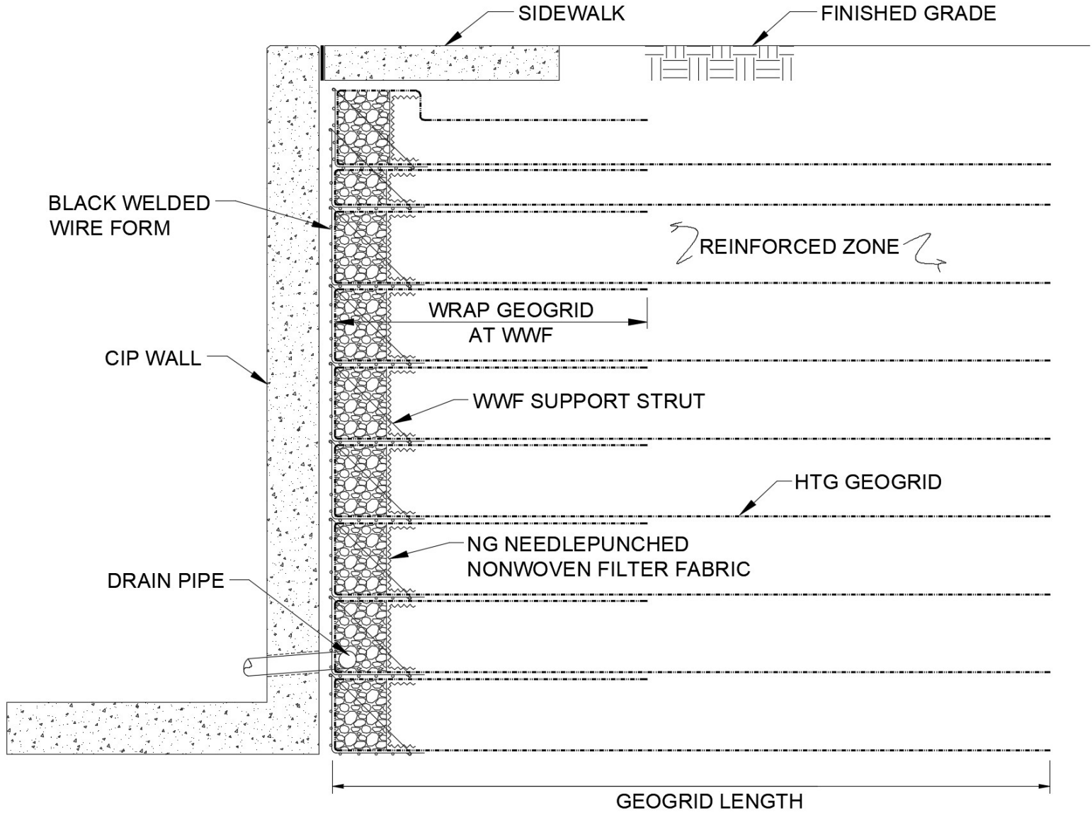
TYPICAL PRESSURE RELIEF WALL CROSS-SECTION
