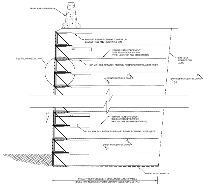
TYPICAL TEMPORARY MSE WALL CROSS-SECTION NOT TO SCALE
