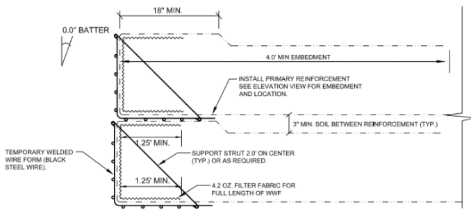
FACING DETAIL NOT TO SCALE
